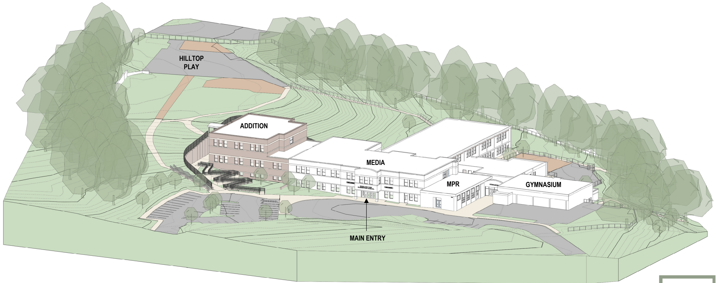
PROPOSED | MASSING VIEW FROM NORTHWEST | SCHOOL BUS LOOP/MAIN ENTRANCE AREA
